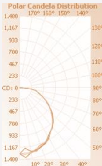
Downlight
